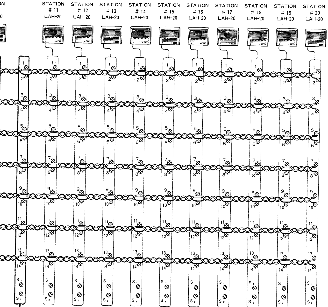
STATION NUMBER CODING SWITCH
