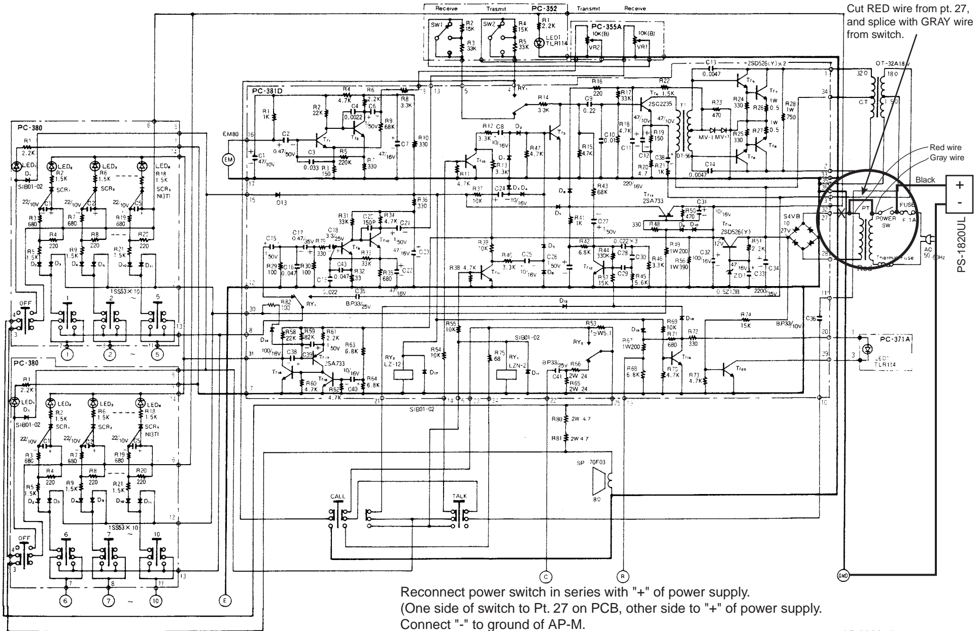
AP-10M Schematic Diagram
