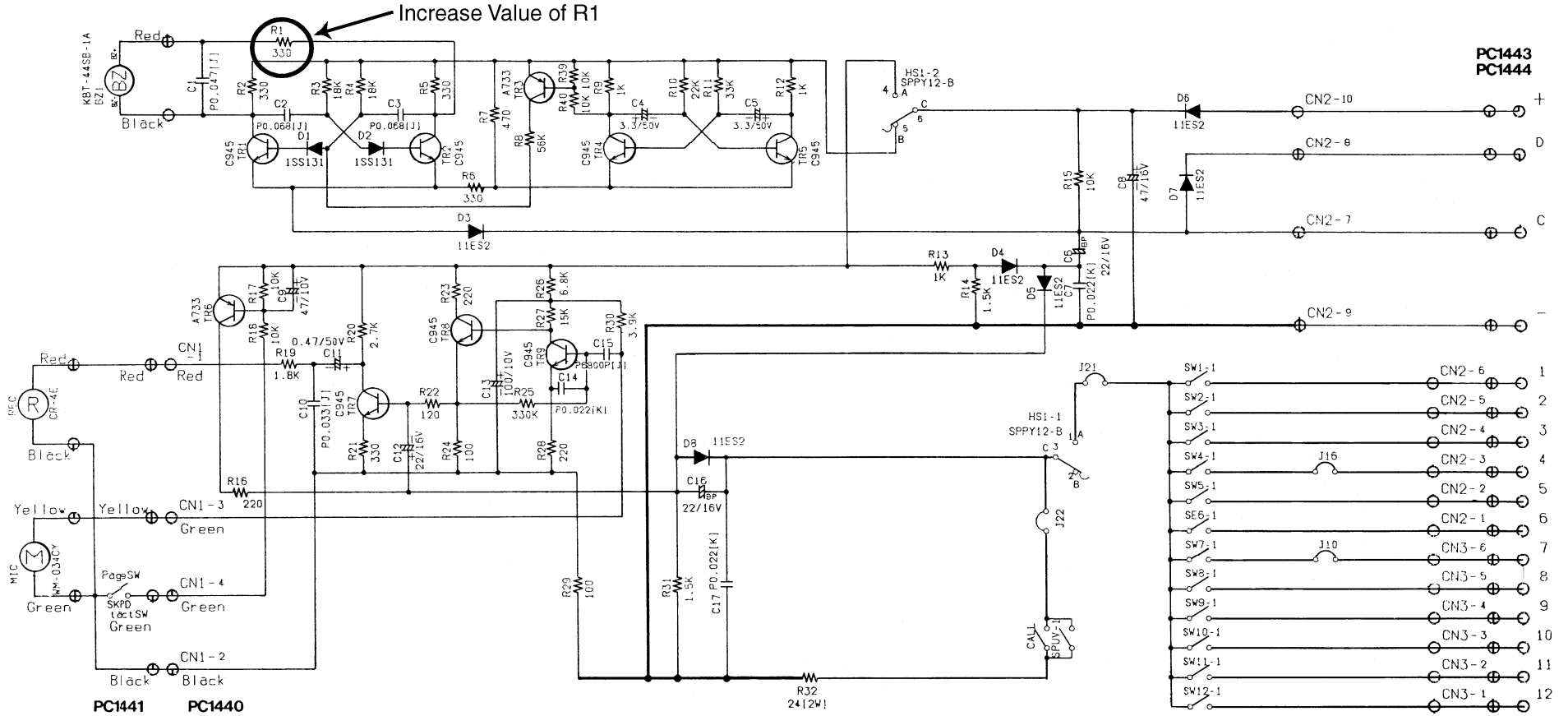
TD-12H/B Schematic Diagram
